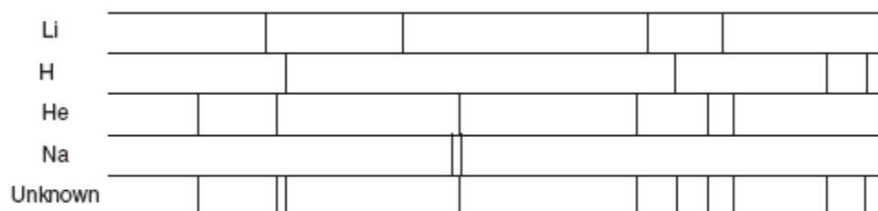
Bright-Line Spectra
